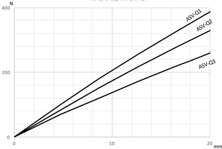
RADYAL / RADIAL
